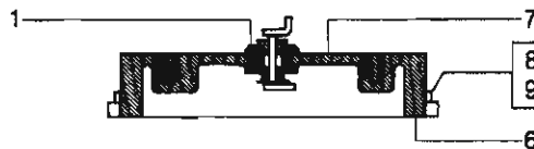
Index Plate Assembly
